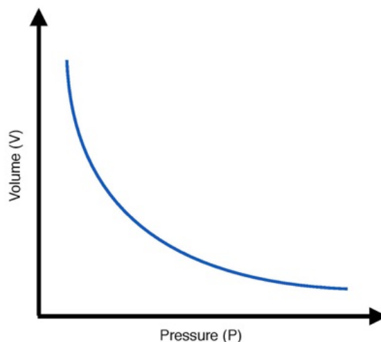
Figure 4: Boyles law
